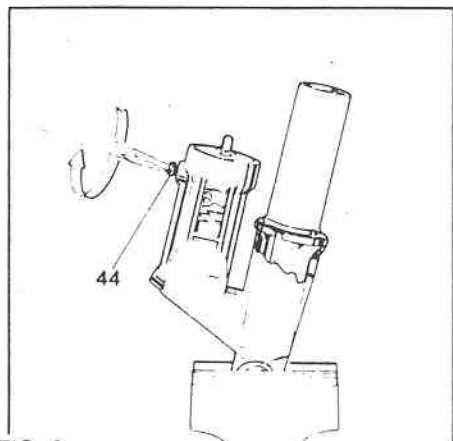
FIG. 6 Now release with a screwdriver (ref. 5) the screw and O-ring (44) paying careful attention to the O-ring. Empty all the oil contained in the shock body and if necessary, clean it with very clean petroleum or methylated spirit.
