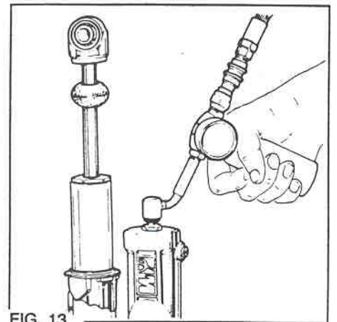
FIG. 13 The reason for pressurizing the bellows is to keep the oil under pressure which will minimize aeration giving more constant damping. It should be remembered that the bellows contain a very small amount of air and therefore widely fluctuating pressure readings will be obtained if normal tyre pressure gauges are used. The best results are obtained by using an in-line pressure gauge which will exactly register the pressure of the contents in the bladder (ref. 93.58).
